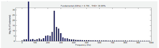
Fig.13. THD without UPQC in source side
