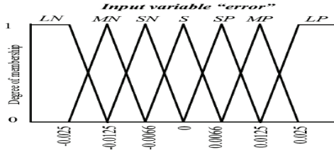
Fig.3.Fuzzification Input voltage variable 1
