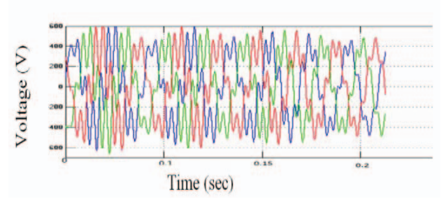
Fig.7. Voltage waveform without UPQC
