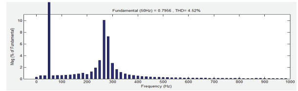
Fig.19. THD with conventional UPQC in load side
